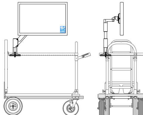
Mag Monitor Arm, Mag HD Thru Desk Mount & Mag HD Thru Desk Support Plate shown with 30" Apple Cinema display mounted on Modified Mag Junior
