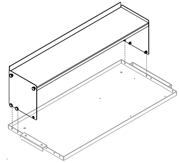
Mag Senior Sound Tray with Mag 24" Top Shelf
