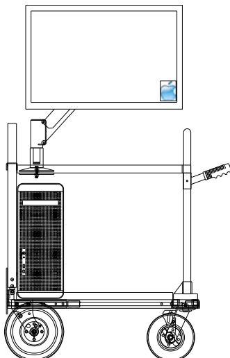
Magliner Mini with Mag LCD Monitor Arm, Mac Pro and 30" Apple Cinema Display (Page 121)
