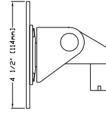
4, 8, 12" Tilt Head to 5/8" Baby Pin Adapter
