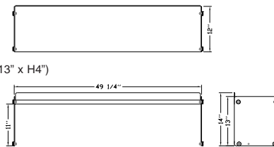
Mag Senior Sound Tray with Mag 18" Top Shelf
